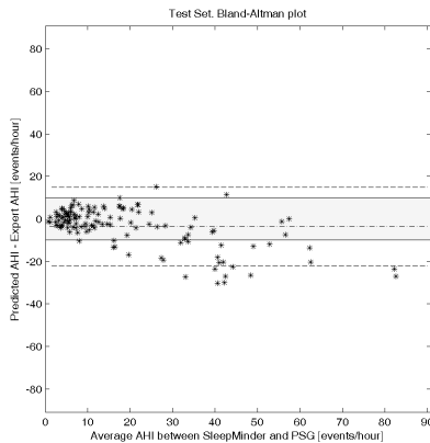
Fig.5. Bland-Altman plot of SleepMinder vs. PSG AHI in the Test Set. The grey sector represents an agreement band of ± 10 events/hour.
